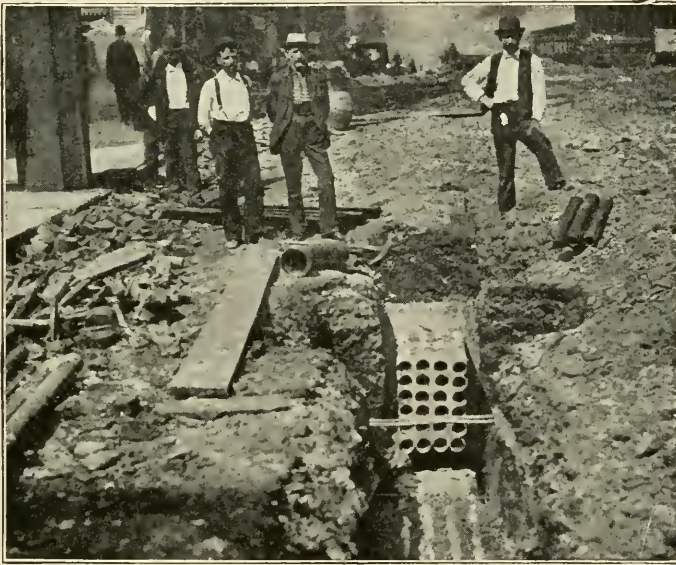
Fig. 48. Cement-Lined, Iron-Pipe Duct System in Course of Construction
